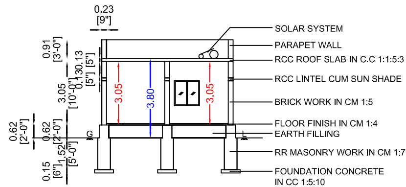
SECTION "AB"
