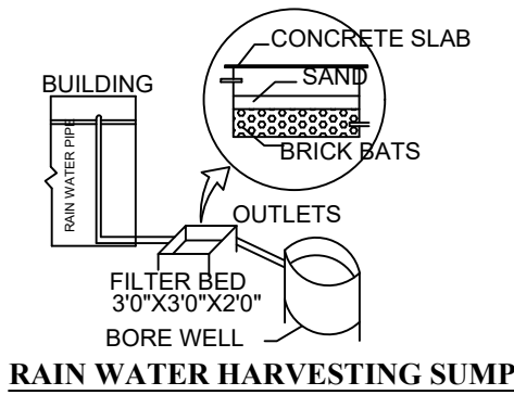
RAIN WATER HARVESTING SUMP
