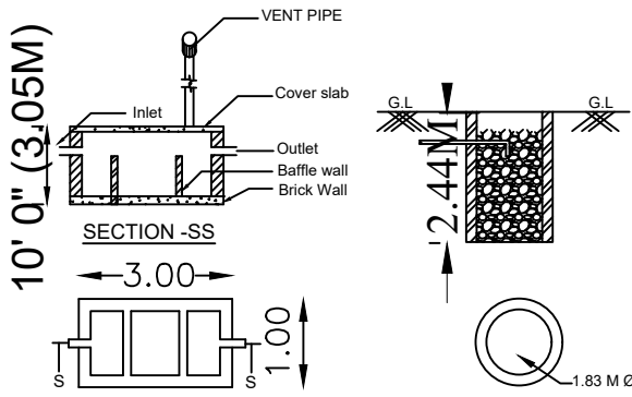
SEPTIC TANK & SOAK PIT DETAILS
