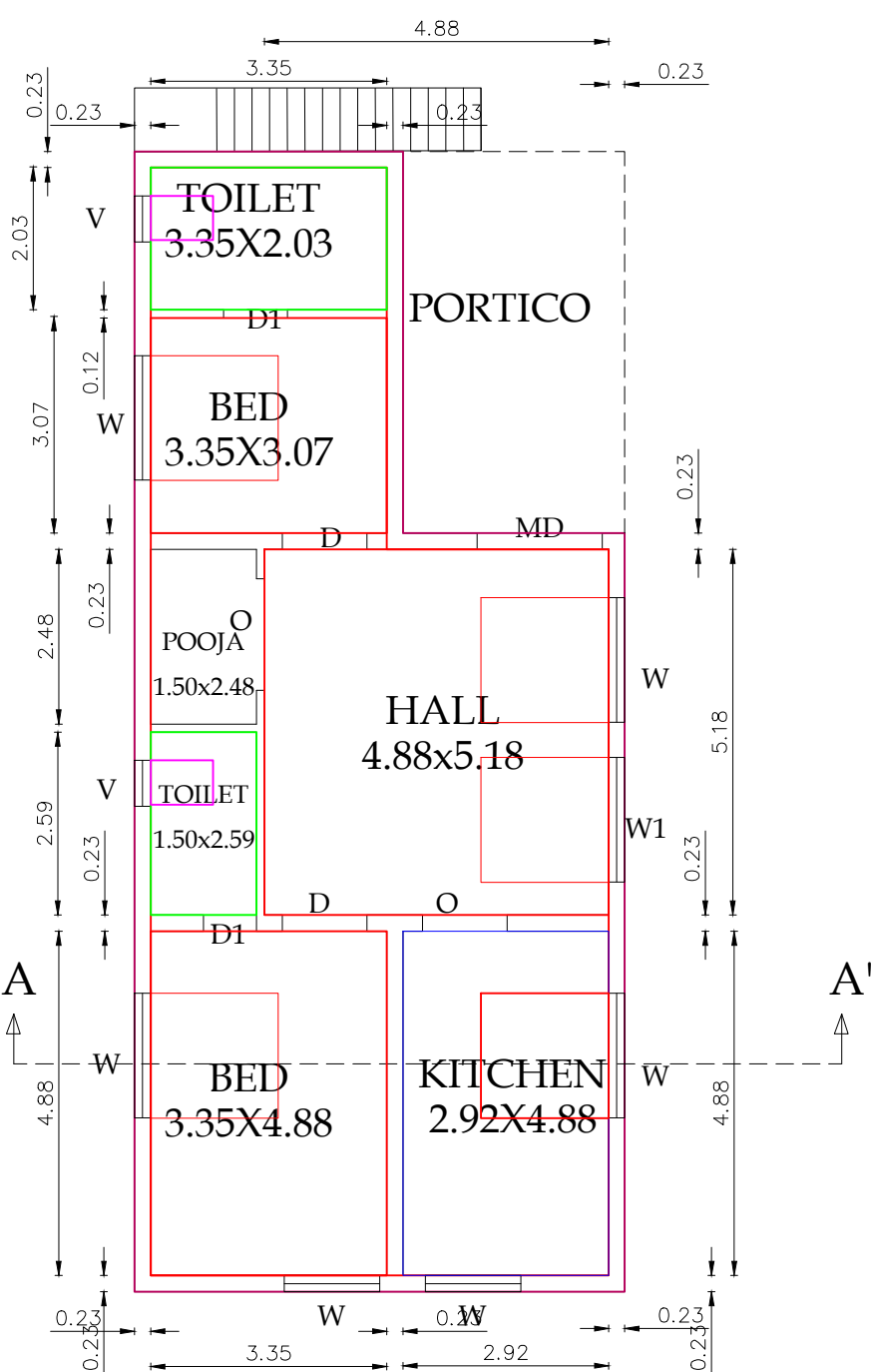
GROUND FLOOR
