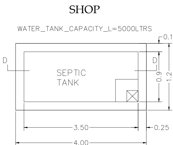
PLAN OF SEPTIC TANK SCALE 1"=2'0"
