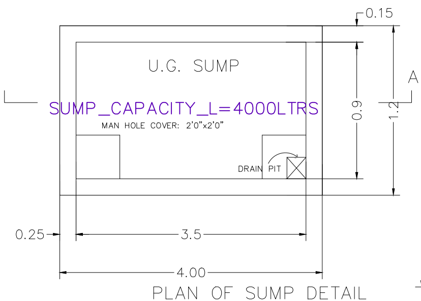
PLAN OF SUMP DETAIL SCALE 1"=4'0"
