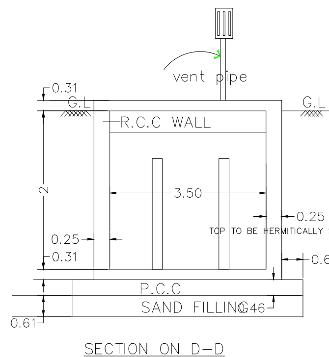
SECTION ON D-D
