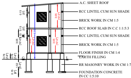
SECTION "AA","BB"
