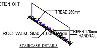
STAIRCASE DETAILS
