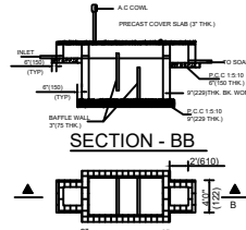
AN OF SEPTIC TANK
