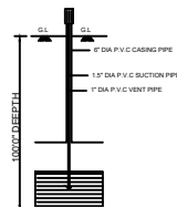
SECTION ON - "AB"
