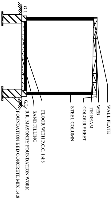
SECTION ON CD
