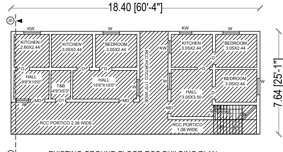
EXISTING GROUND FLOOR RCC BUILDING PLAN DOOR NO'S:7/1,7/2,7/3, ASS.NO'S:6054,6055,6056,.
