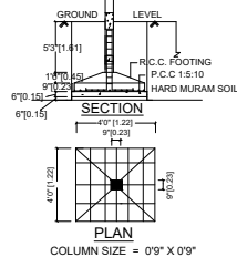
FOUNDATION DETAILS
