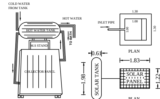
SOLAR WATER HEATER SYSTEM
