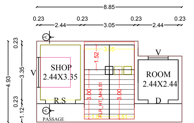
PROPOSED GF.PLAN
