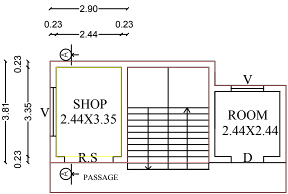
PROPOSED FF.PLAN
