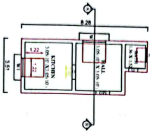
PROPOSED GROUND FLOOR PLAN
