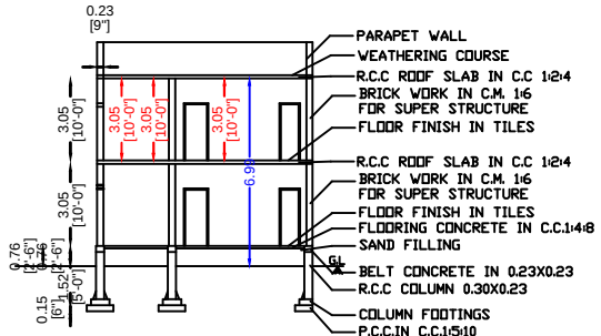
SECTION "PS"
