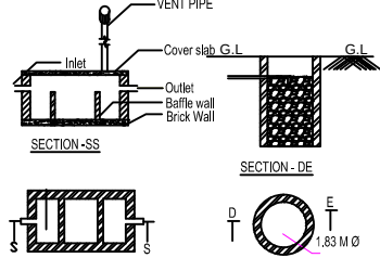
SEPTIC TANK & SOAK PIT DETAILS
