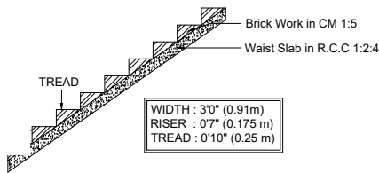
STAIRCASE DETAILS
