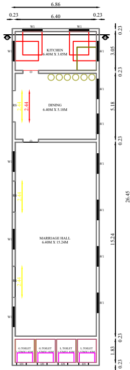
PROPOSED GROUND FLOOR PLAN
