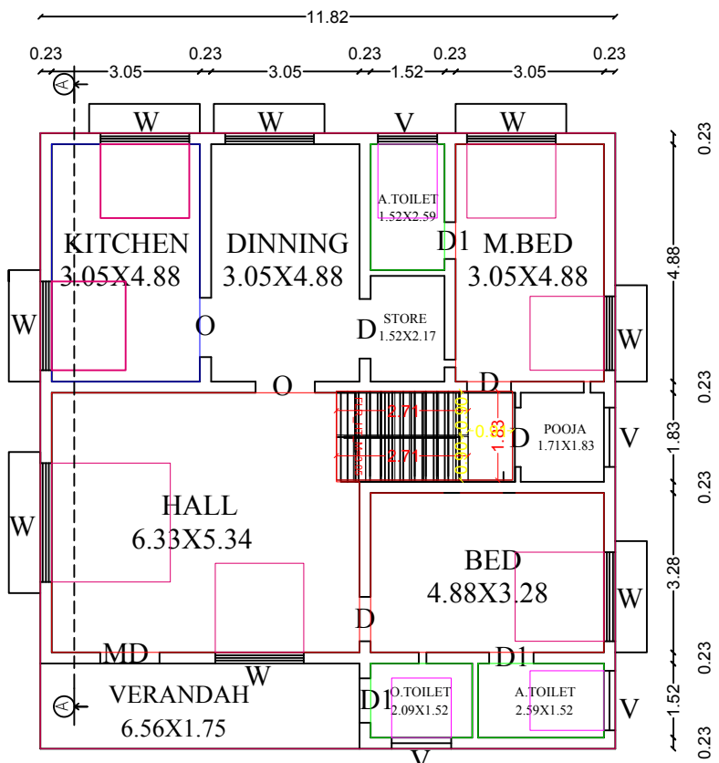
PROPOSED.GF.PLAN
