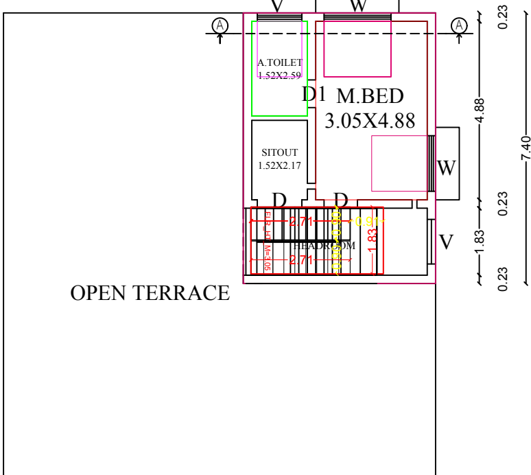
PROPOSED.FF.PLAN
