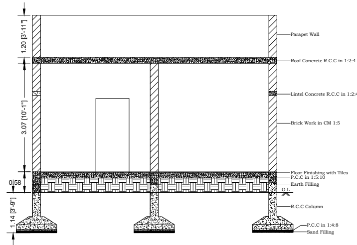
SECTION X-X
