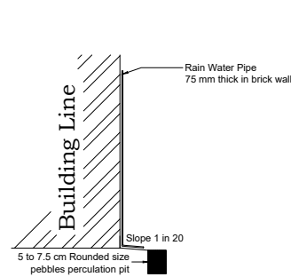
RAINWATER HARVESTING
