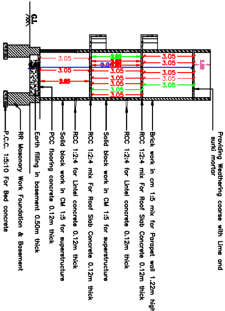
SECTION ON 'AB'
