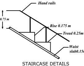
STAIRCASE DETAILS
