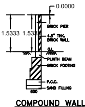
COMPOUND WALL
