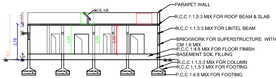
SECTION A-A FROM NORTH
