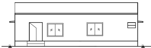
ELEVATION ON NORTH
