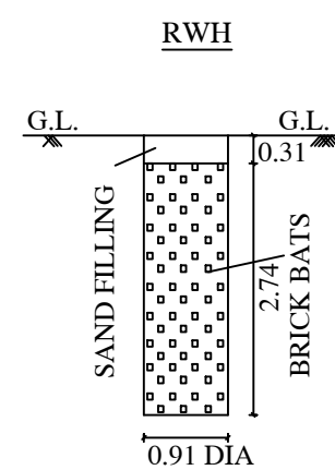
SECTION ON " A-B "
