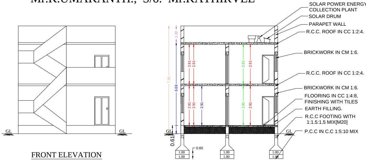
FRONT ELEVATION
