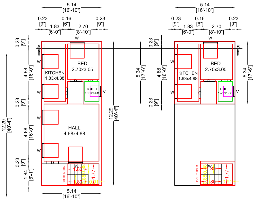
ST FLOOR PLAN
