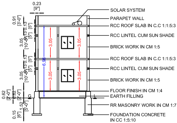
SECTION "AB"
