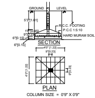
FOUNDATION DETAILS
