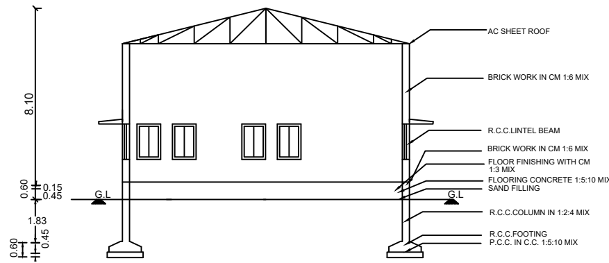
SECTION ON "PP"
