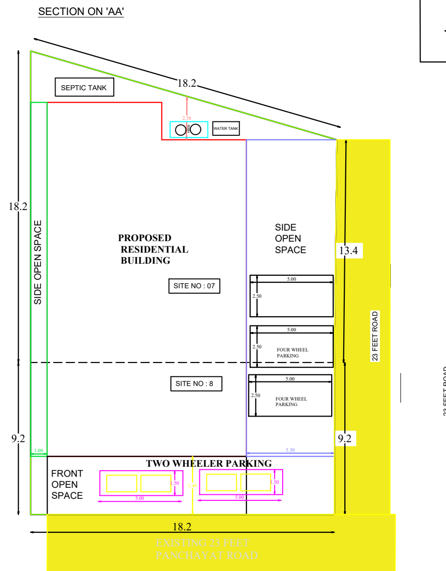
SITE & LOCATION PLAN SCALE - 1 : 800
