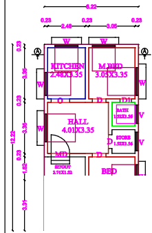
PROPOSED GROUND FLOOR
