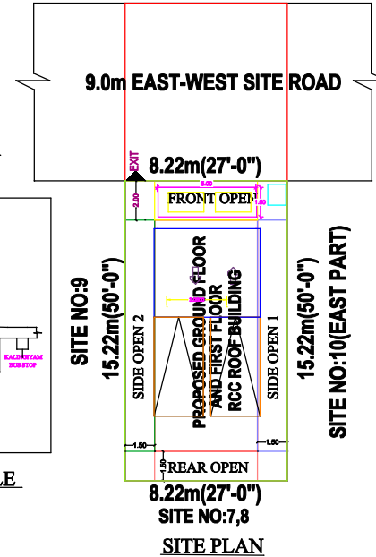
SITE PLAN
