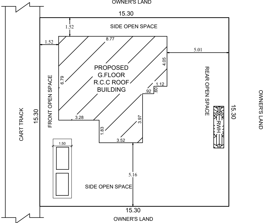
SITE PLAN SCALE 1CM:1M
