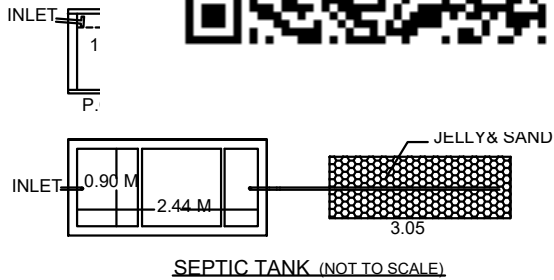
SEPTIC TANK (NOT TO SCALE)
