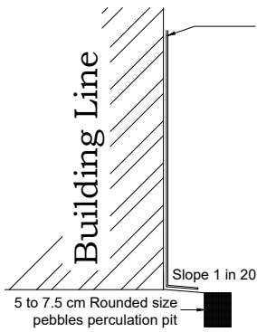
RAINWATER HARVESTING
