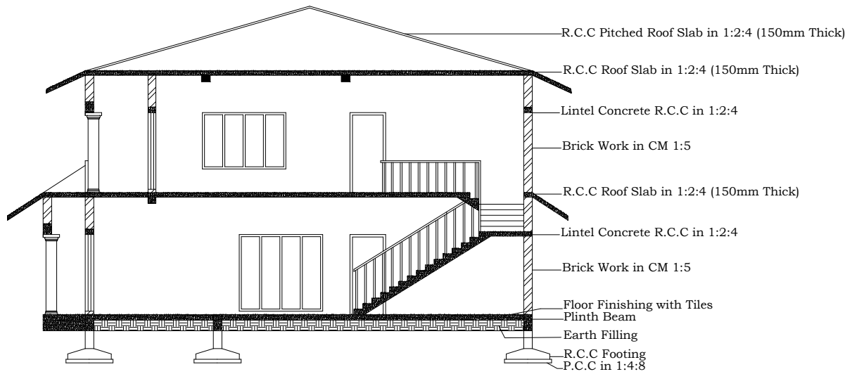
SECTION X-X
