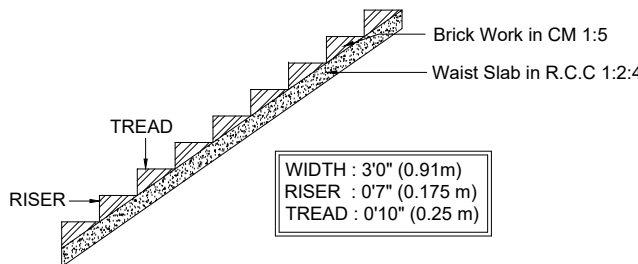
STAIRCASE DETAILS
