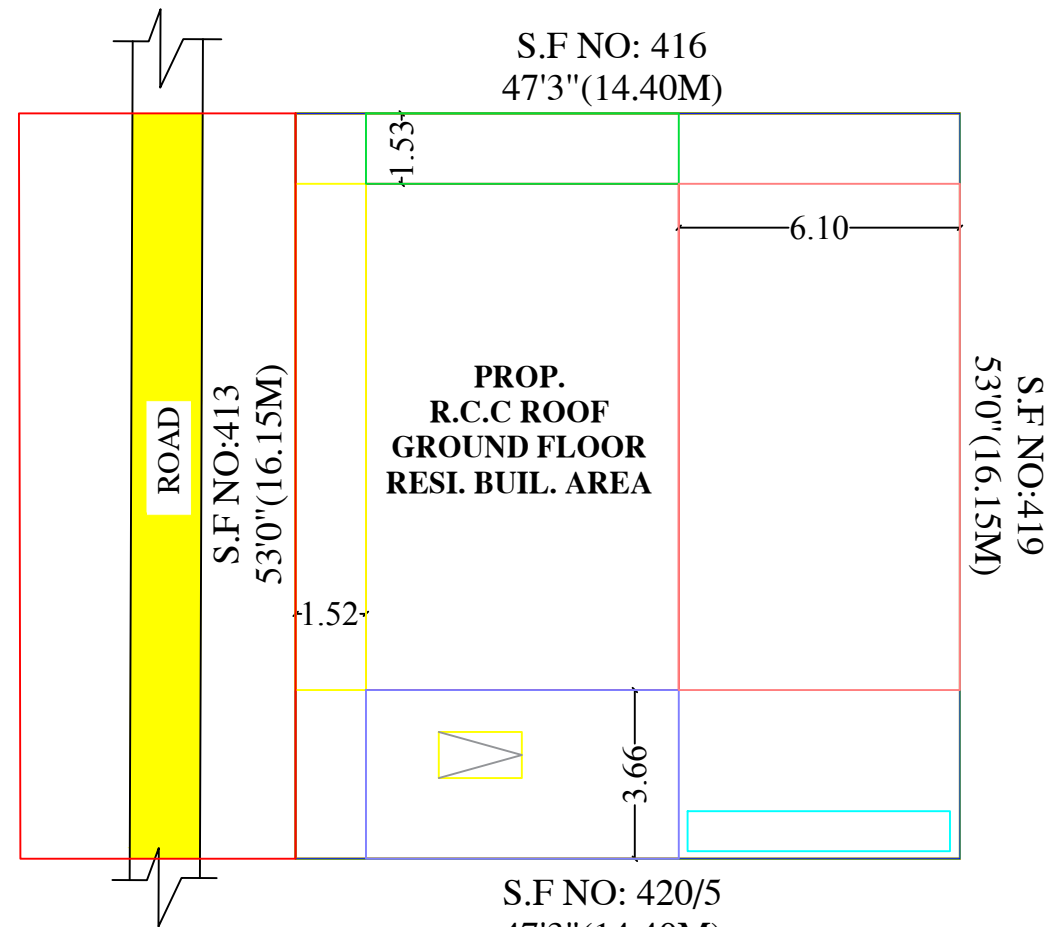
SITE PLAN
