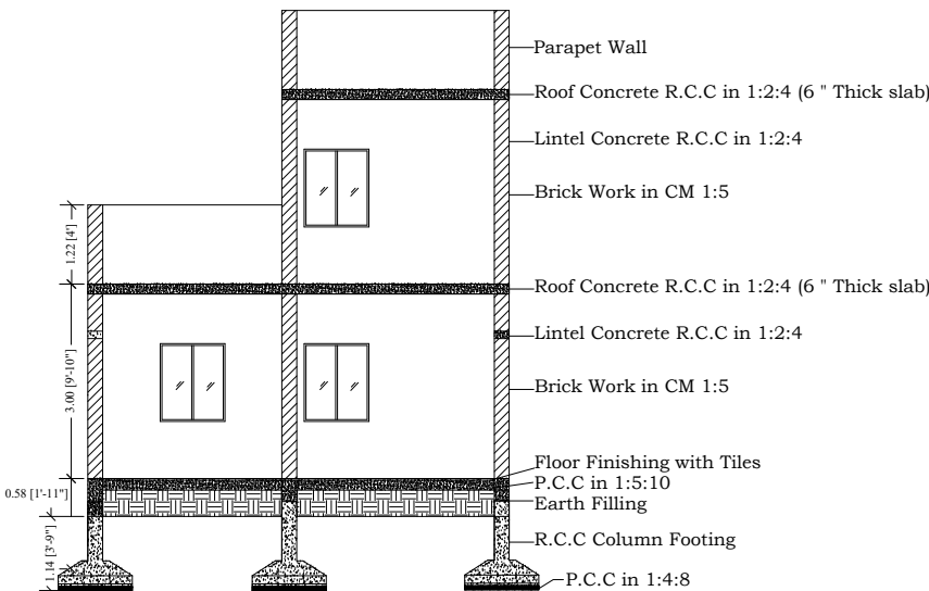
SECTION X-X
