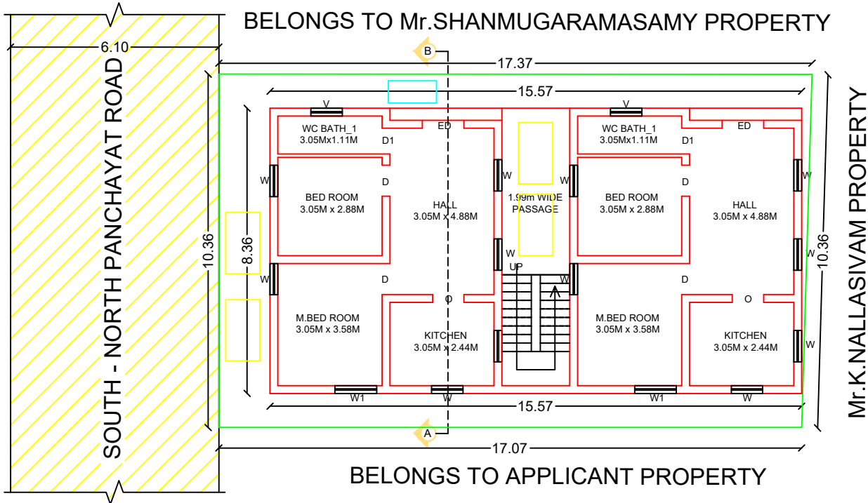
SITE PLAN CUM GROUND FLOOR PLAN
