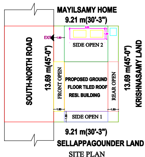
SITE PLAN
