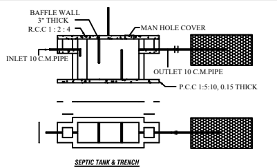
SEPTIC TANK & DRAINAGE
