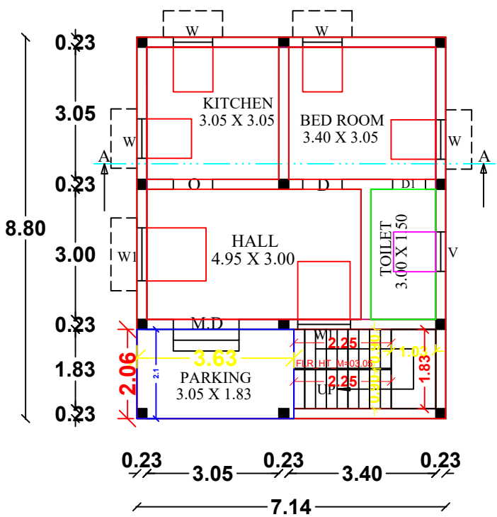
GROUND FLOOR PLAN ( North Facing )
