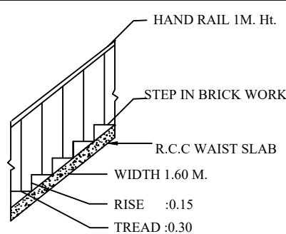
STAIR DETAIL
