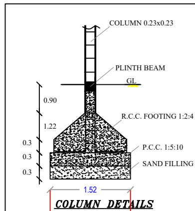
COLUMN DETAILS
