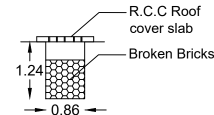
Rainwater Harvesting pit (Not to Scale)
