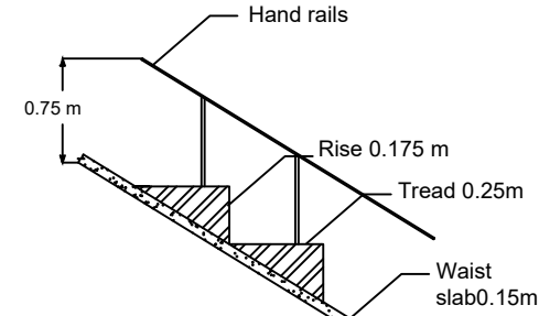
STAIRCASE DETAILS (Not to Scale)
