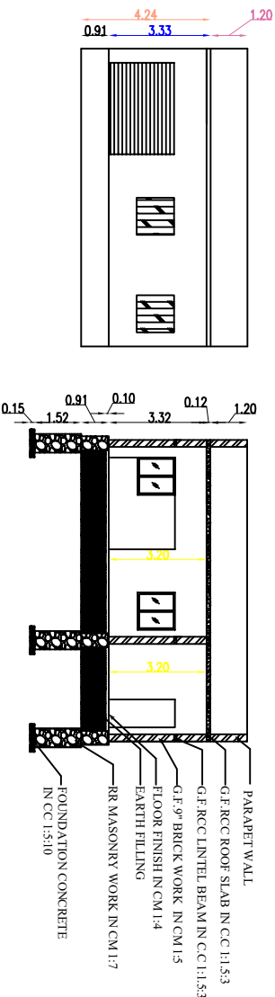
SECTION ON A-A
