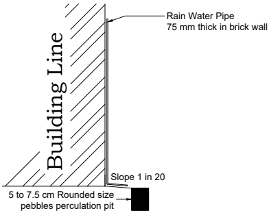
RAINWATER HARVESTING
