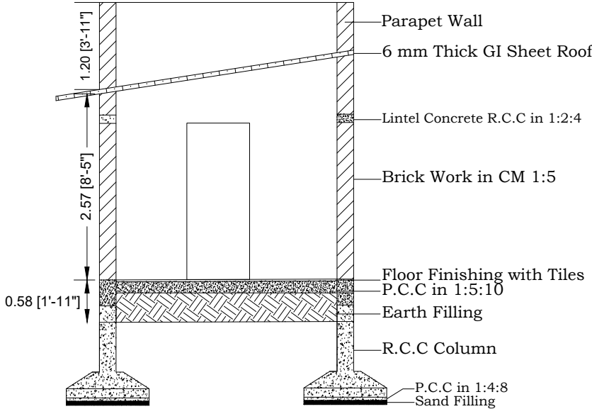
SECTION X-X
