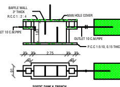
SEPTIC TANK & TRENCH
