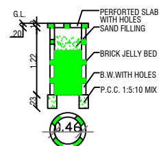
RAIN WATER HARVEST
