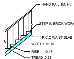
STAIR DETAIL
