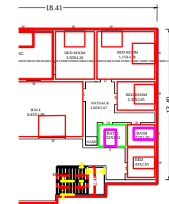
FIRST FLOOR PLAN SCALE 1:100
