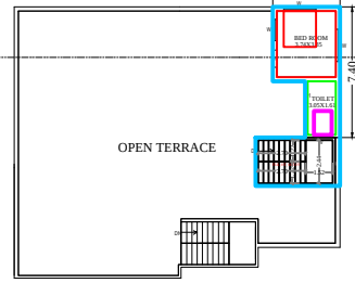
SECOND FLOOR PLAN SCALE 1:100
