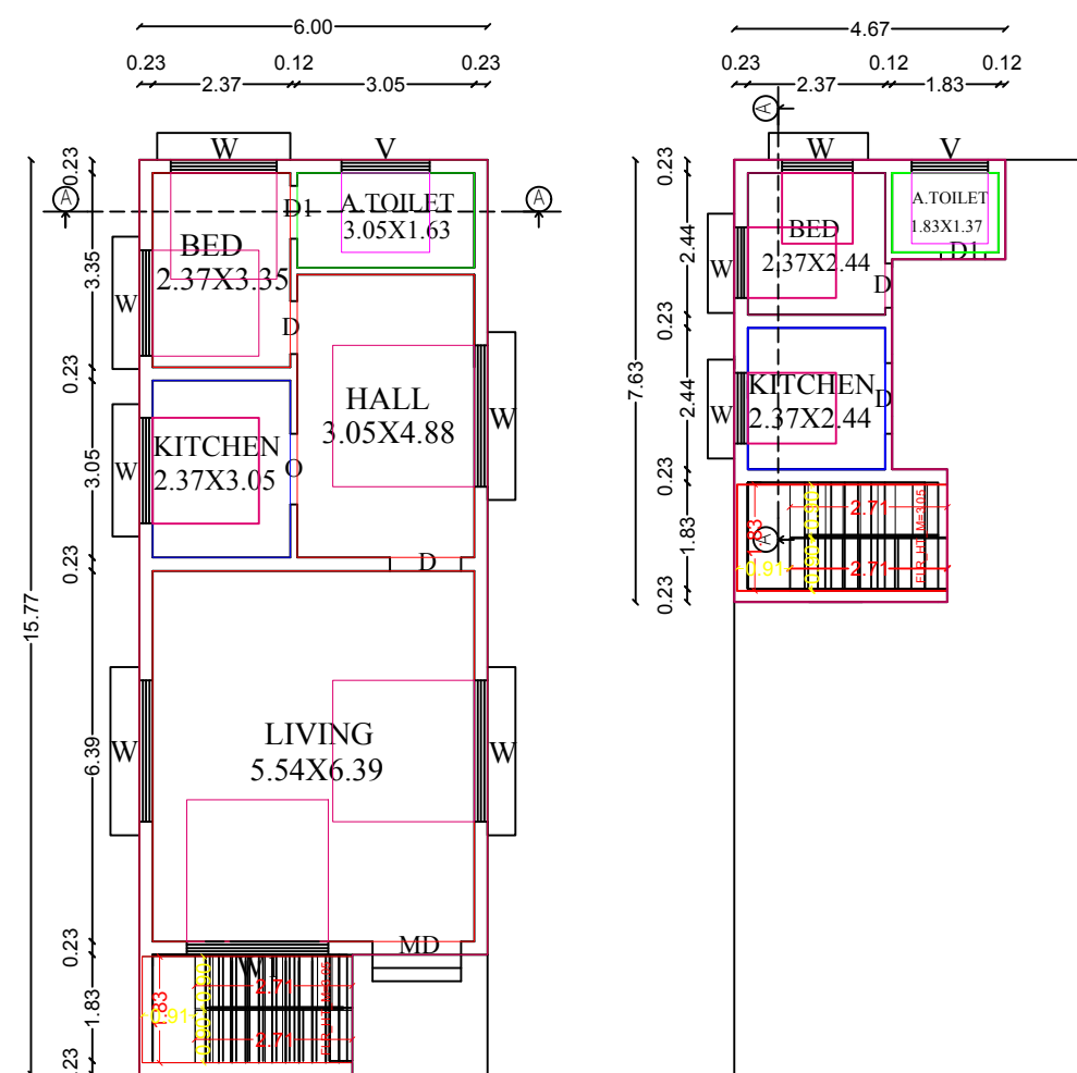
PROPOSED.GF.PLAN PROPOSED.FF.PLAN
