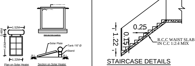
STAIRCASE DETAILS
