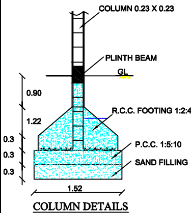
COLUMN DETAILS
