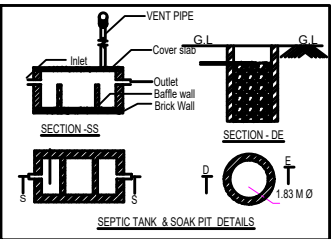
SEPTIC TANK & SOAK PIT DETAILS
