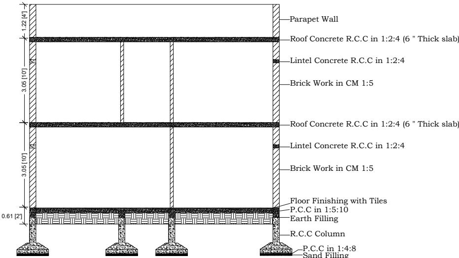
SECTION X-X
