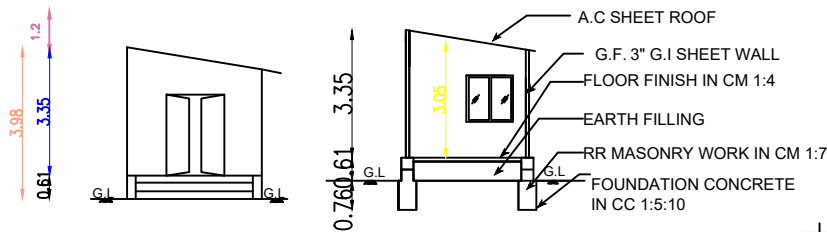
ELEVATION SECTION ON AA
