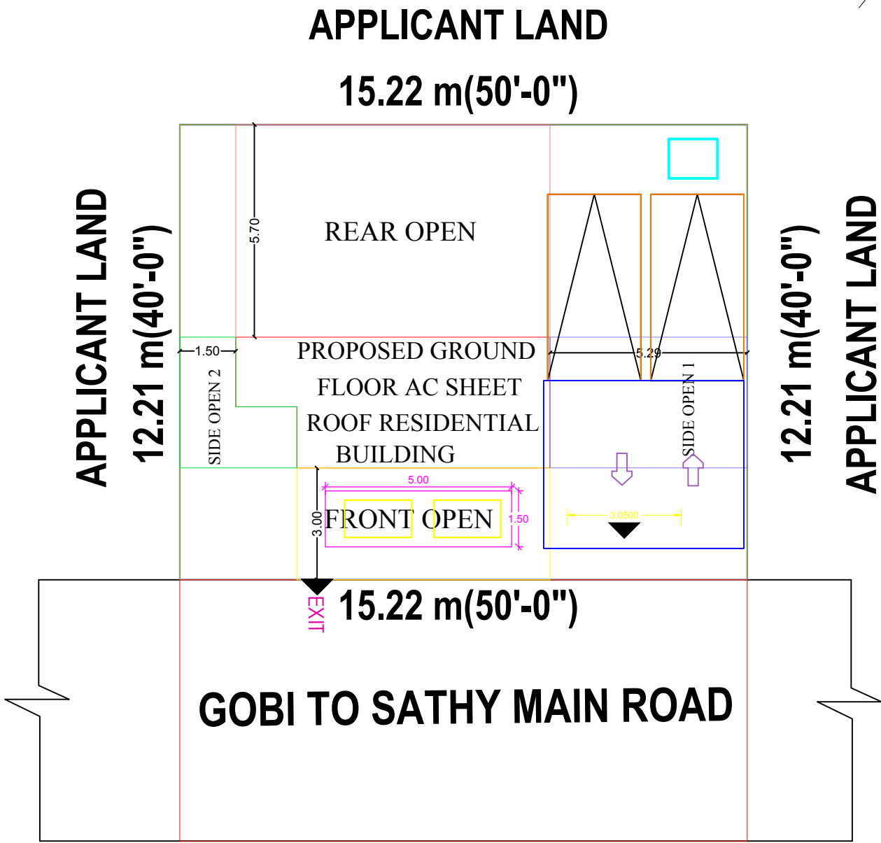
SITE PLAN
