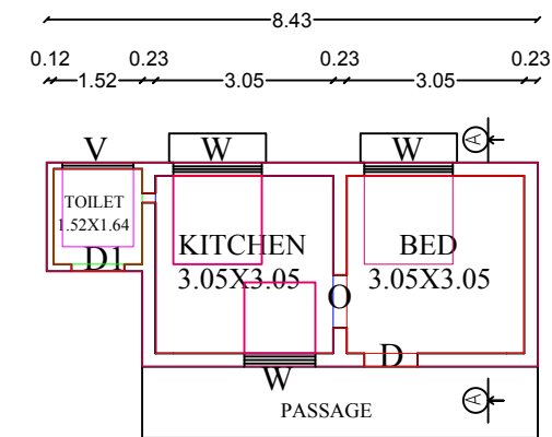
PROPOSED GF.PLAN
