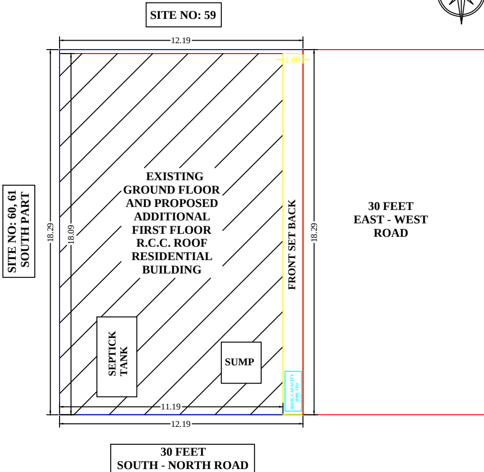
SITE PLAN
