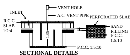
SECTIONAL DETAILS
