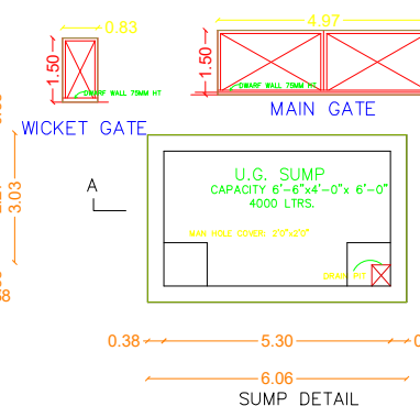
SUMP DETAIL
