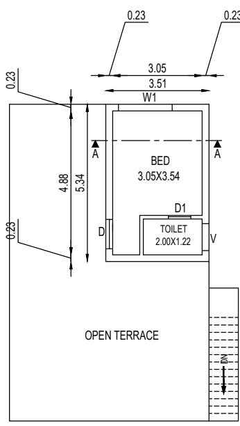
FIRST FLOOR PLAN ( Scale : 1:100)
