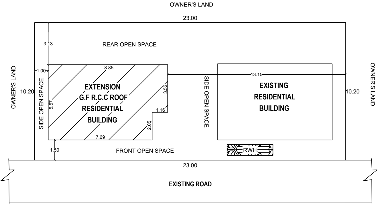
SITE PLAN
