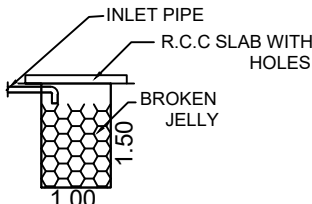
RAIN WATER HARVESTING FILTER BED
