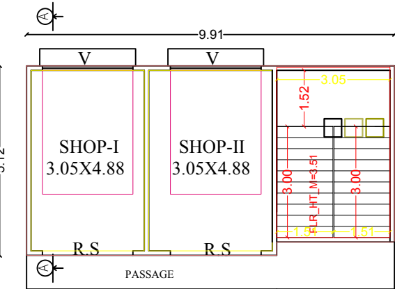
PROPOSED GF.PLAN
