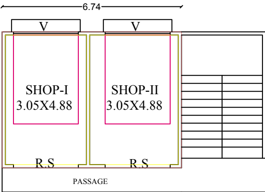
PROPOSED FF.PLAN
